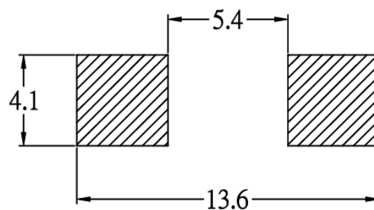
Recommend Land Pattern Dimensions
